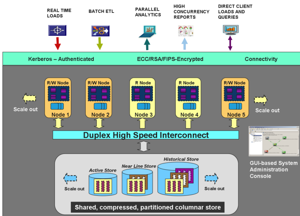
Figure 1: Sybase IQ 15 architecture
